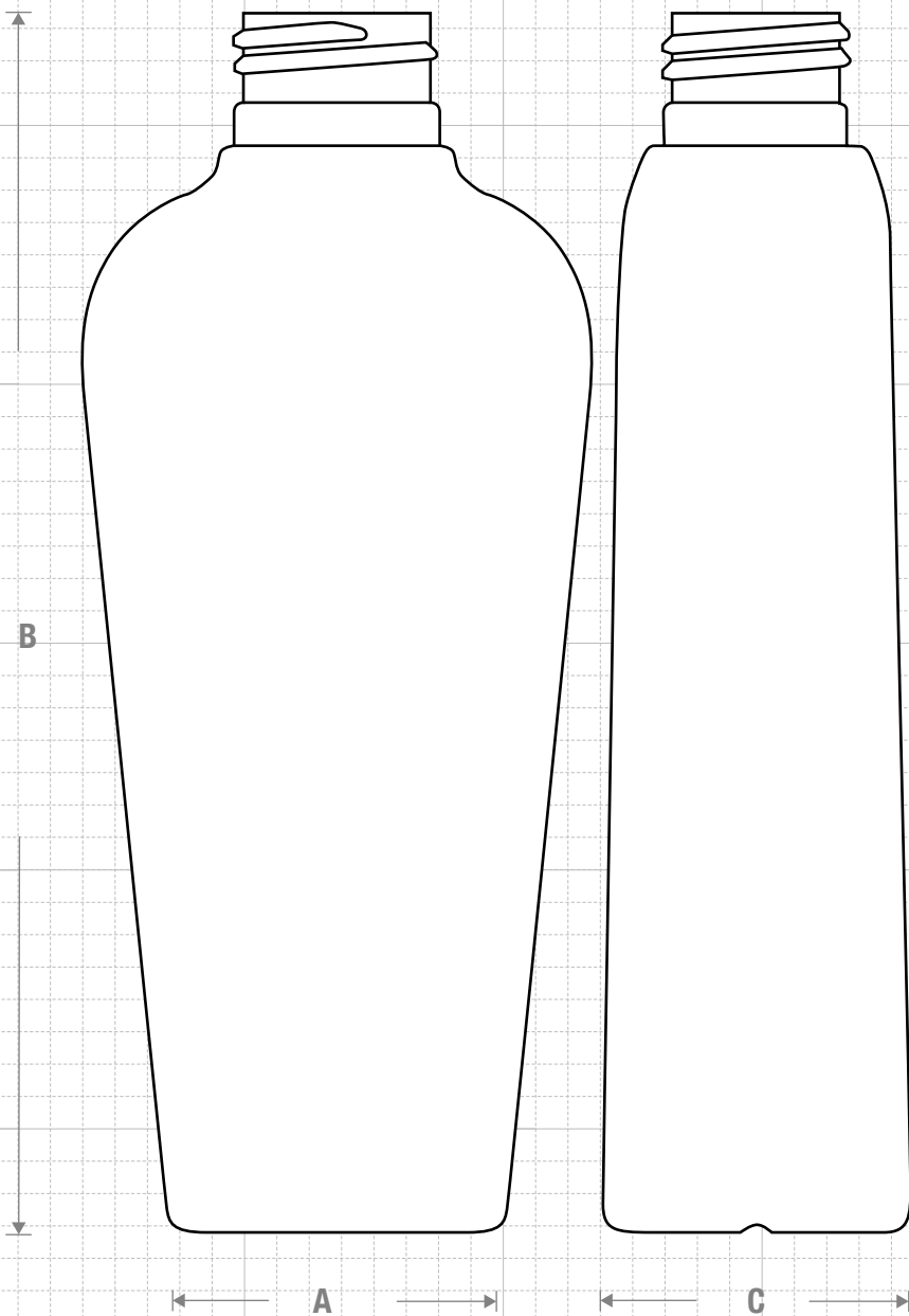
FRONT VIEW
