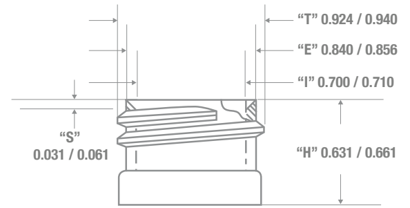
NECK & THREAD DETAIL
