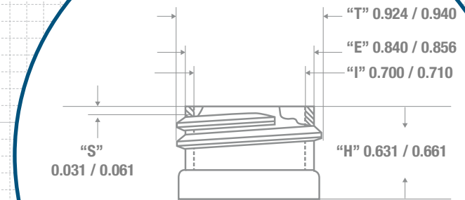
NECK & THREAD DETAIL
