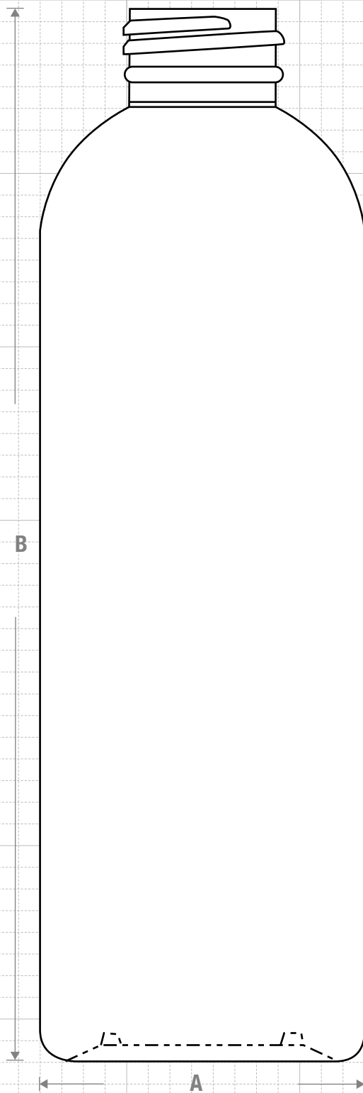
FRONT VIEW
